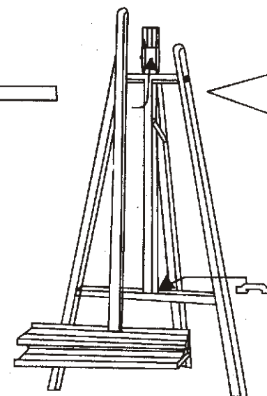
Screw: 4mm×40mm×2pos
